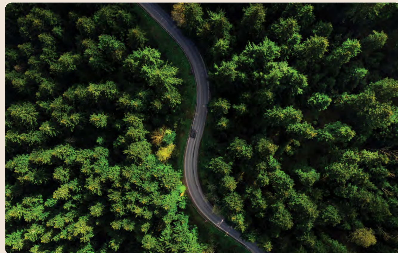
Telstra greenhouse gas emissions
